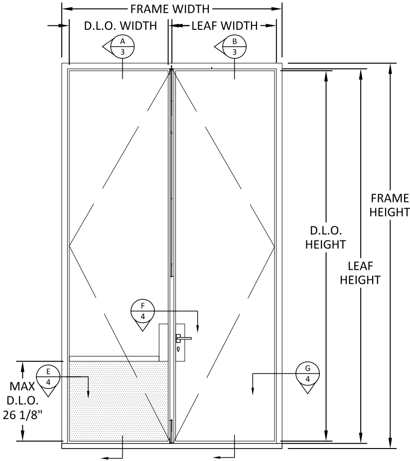
ELEVATION XX FARO 65
