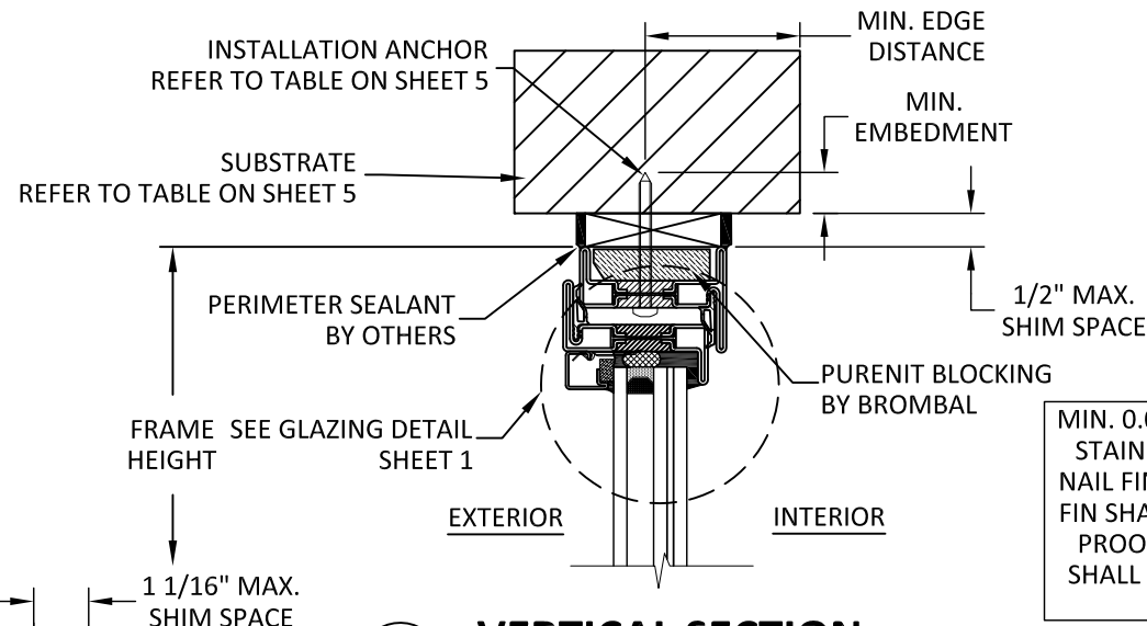
K5 VERTICAL SECTION THROUGH FRAME ANCHOR TYP. INSTALLATION - HEAD/JAMB/SILL
