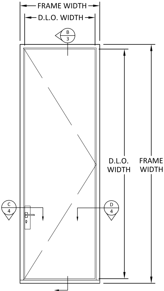
ELEVATION X FARO 65
