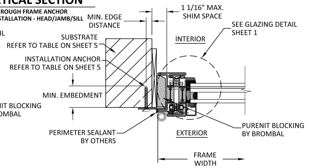
I5 HORIZONTAL SECTION NAIL FIN INSTALLATION TYP. INSTALLATION - HEAD/JAMB/SILL
