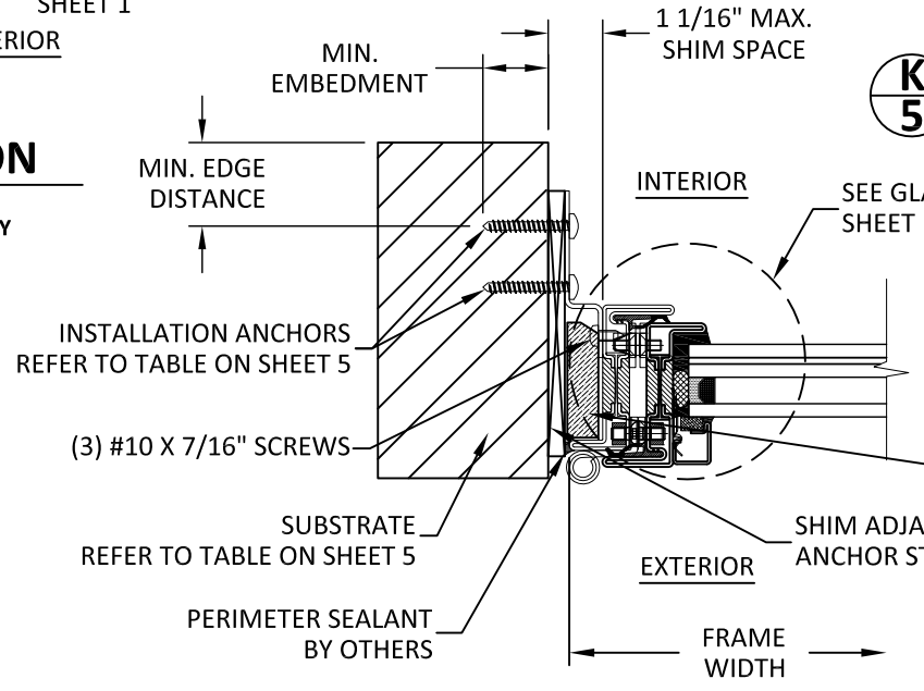
J5 HORIZONTAL SECTION THRU STRAP INSTALLATION TYP. INSTALLATION - HEAD/JAMB/SILL
