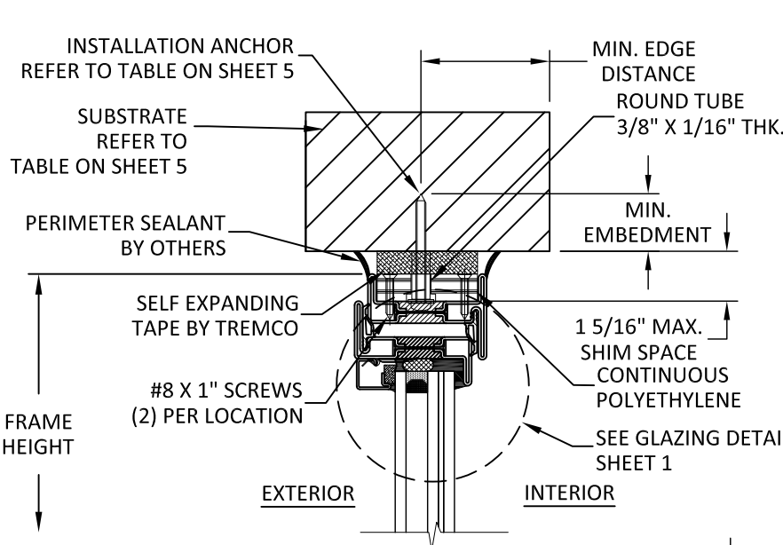
H5 VERTICAL SECTION DEFLECTION ANCHOR TYP. INSTALLATION - HEAD ONLY
